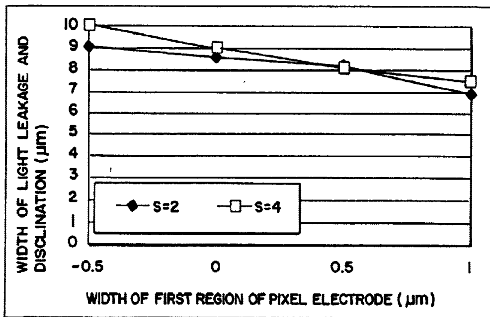
THE RELATION BETWEEN WIDTH OF FIRST REGION OF PIXEL ELECTRODE AND WIDTH OF DISCLINATION AND LIGHT LEAKAGE DISTANCE BETWEEN PIXEL ELECTRODES: 2.0 \mu\text{m} (s=2), 4.0 \mu\text{m} (s=4)
