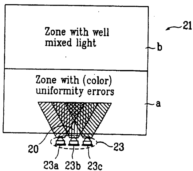
FIG. 4 Related Art
