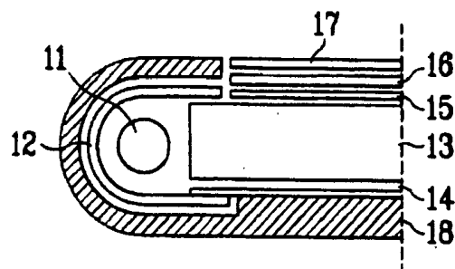
FIG. 3 Related Art
