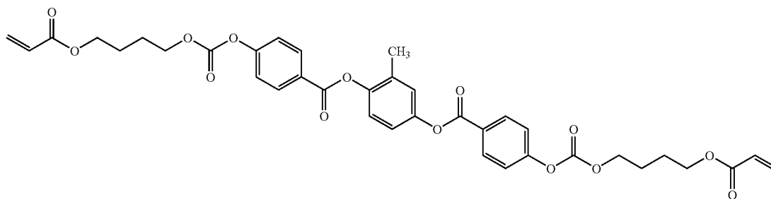
Rod-like liquid crystalline compound A
