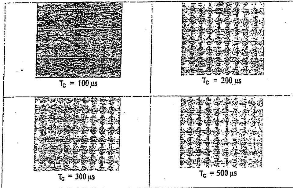
Figure 22 : Optical state of the pixels of a 160x480 display according to the prior art ("parallel" brushing) as a function of the duration of the column voltage addressed by the signals defined in Table II: "on" (light) T texture; "off" (dark) U texture.
