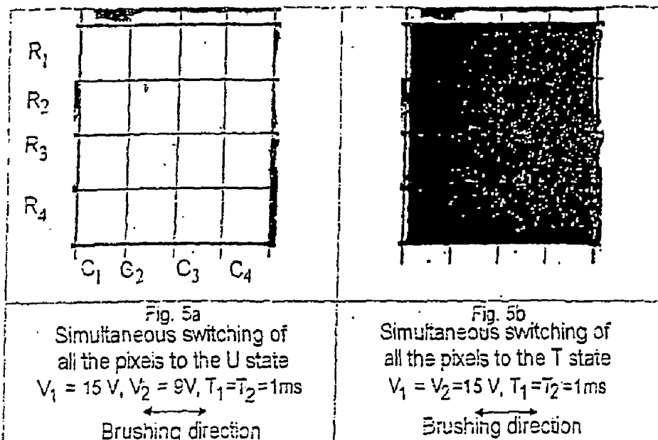
Figure 5 : Simultaneous switching of all the pixels to the U (white) state or T (black) state.
