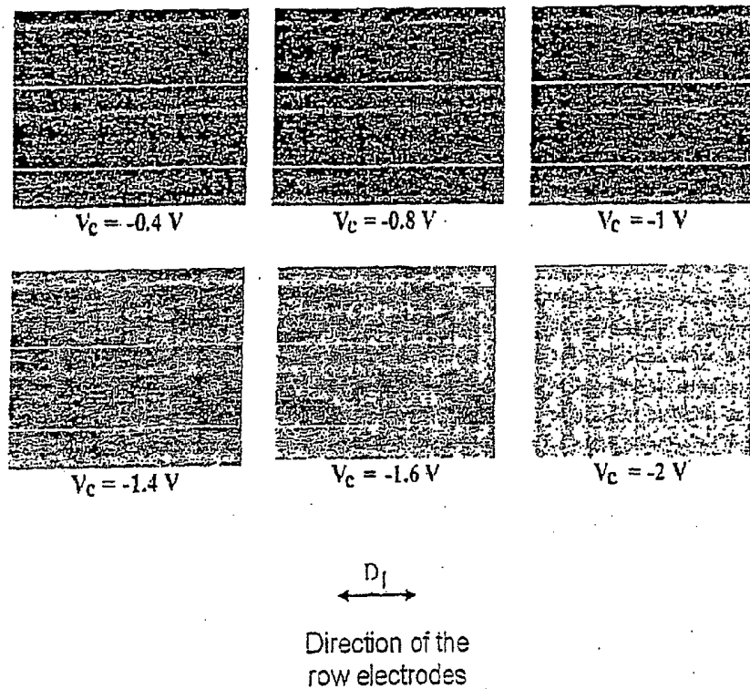
Figure 21 : Optical state of the pixels of a 160x480 display according to the prior art ("parallel" brushing) as a function of the column voltage addressed by the signals defined in Table I: "on" (light) T texture; "off" (dark) U texture
