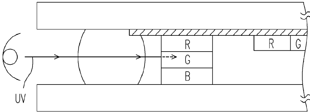
FIG. 3 (PRIOR ART)
