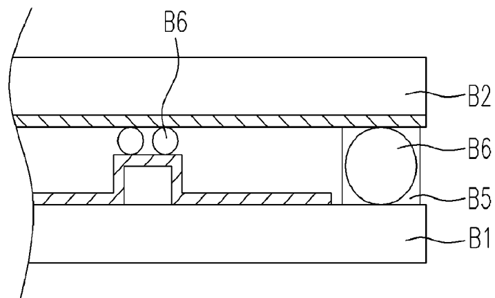
FIG. 5 (PRIOR ART)
