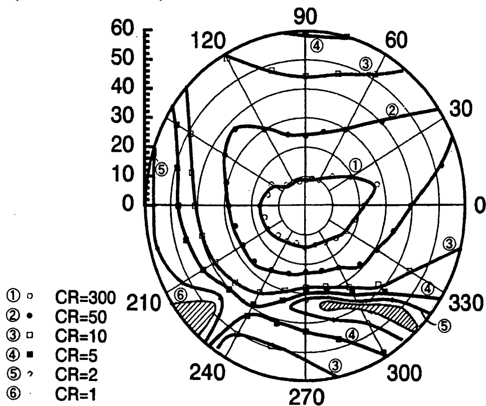
FIG. 12 (PRIOR ART)
