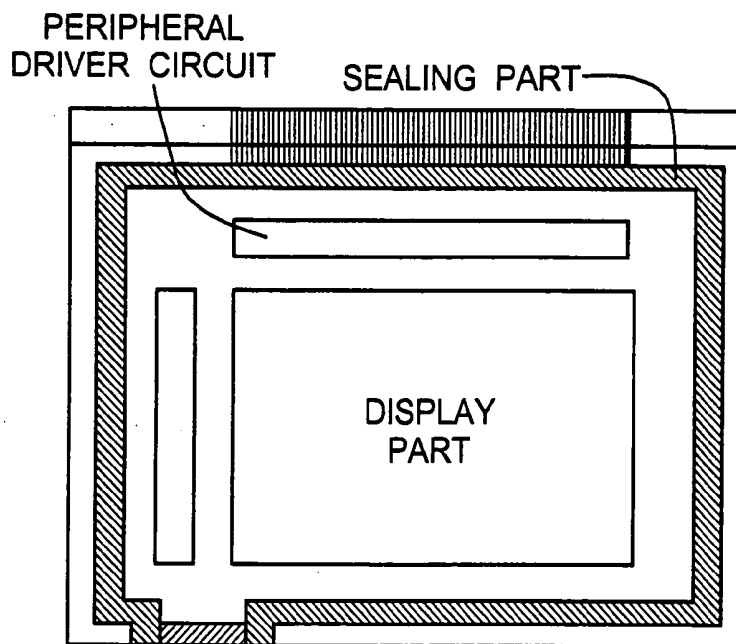
STRUCTURE OF CONVENTIONAL PANEL
