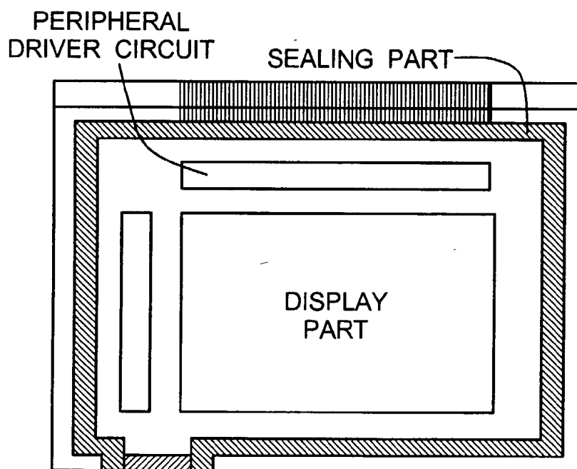
STRUCTURE OF CONVENTIONAL PANEL
