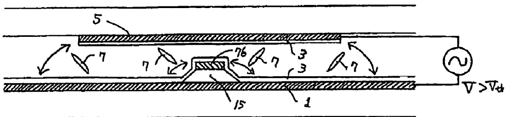
Fig. 57 (Prior Art)
