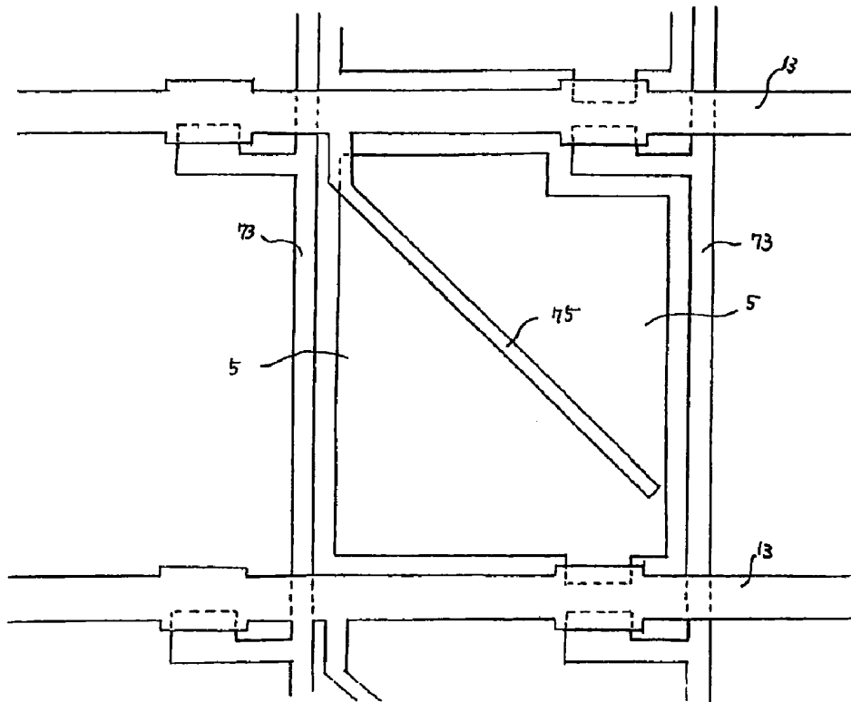
Fig. 54 (Prior Art)
