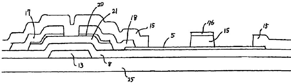
Fig. 58 (Prior Art)
