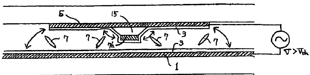
Fig. 56 (Prior Art)
