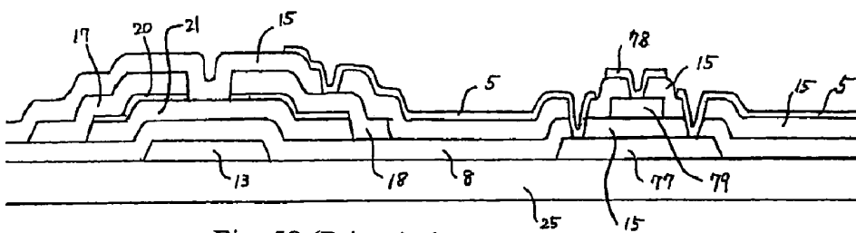
Fig. 59 (Prior Art)
