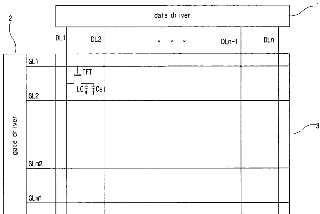
FIG. 2 RELATED ART
