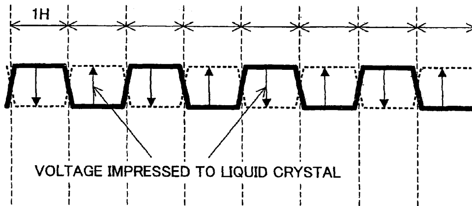
FIG. 12 PRIOR ART
