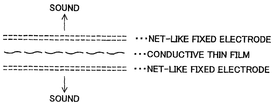
FIG. 13 PRIOR ART
