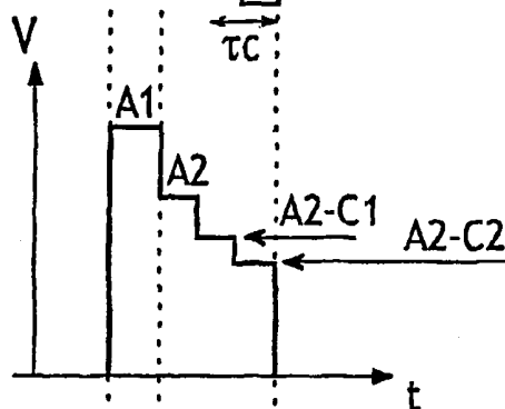
U switch pixel signal FIG. 9d
