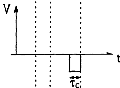
T switch column signal FIG.7c
