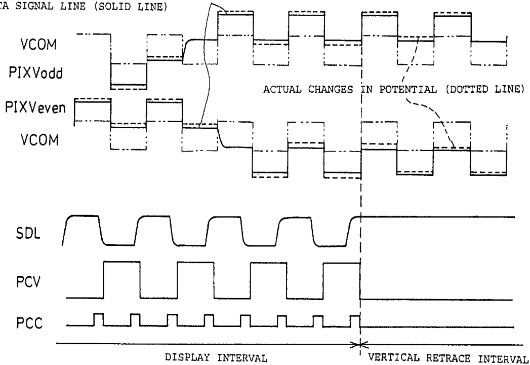
FIG.14 PRIOR ART
