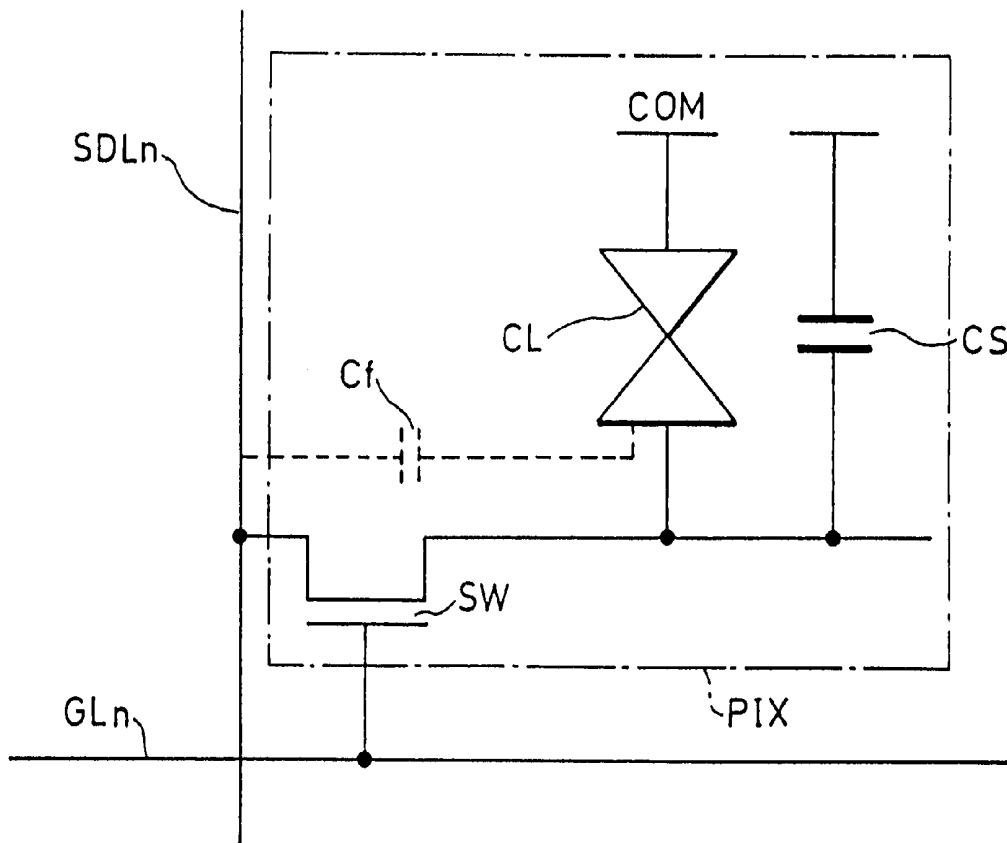
FIG. 12 PRIOR ART
