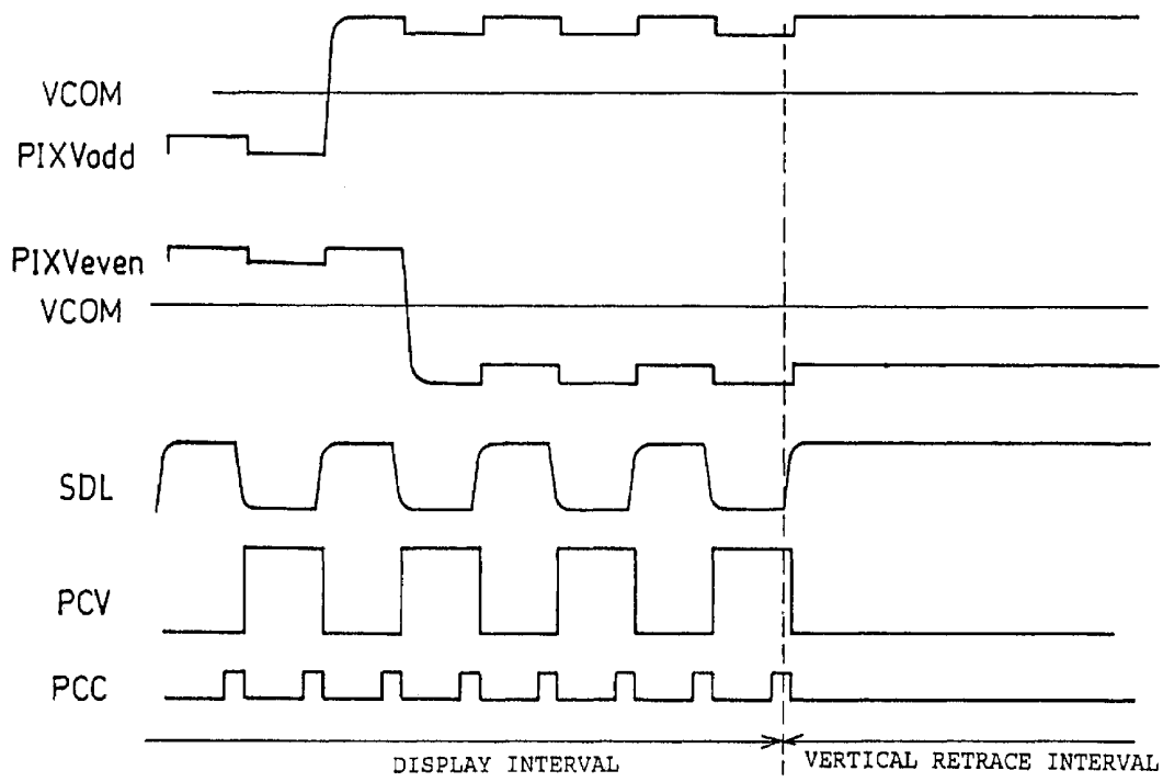
FIG. 13 PRIOR ART
