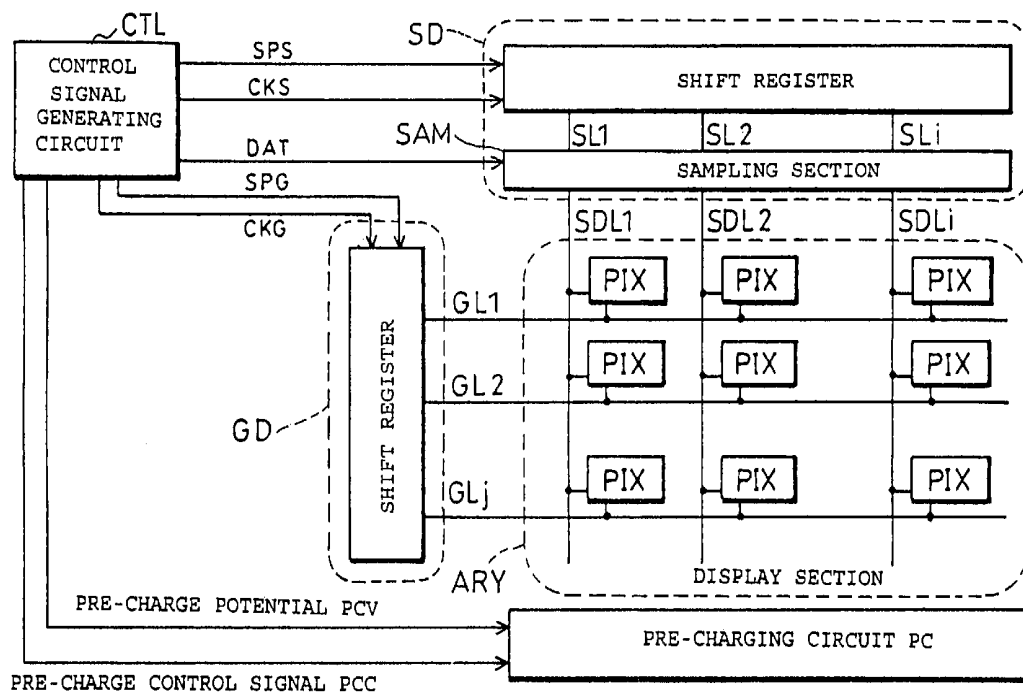
FIG. 11 PRIOR ART
