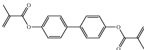
[Chemical Formula 12]
