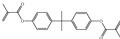
[Chemical Formula 20]
