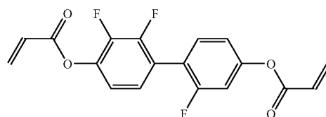
[Chemical Formula 17]
