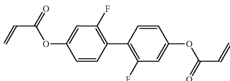
[Chemical Formula 15]
