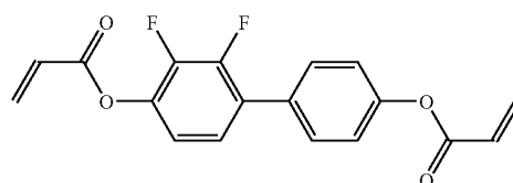
[Chemical Formula 19]
