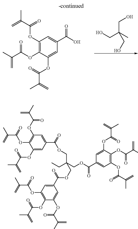
[Reaction Formula 9]
