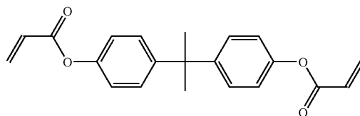
[Chemical Formula 21]
