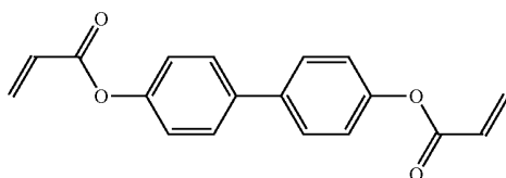
[Chemical Formula 14]
