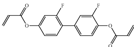
[Chemical Formula 15]
