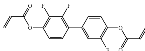
[Chemical Formula 18]
