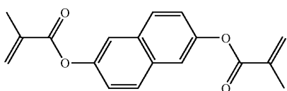
[Chemical Formula 11]
