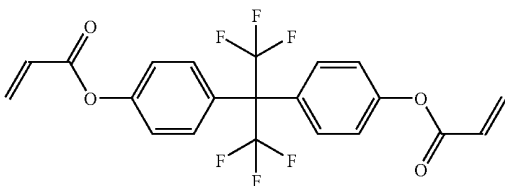
[Chemical Formula 21]
