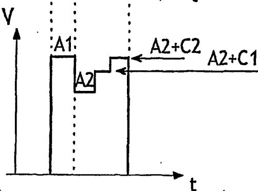
T switch pixel signal FIG.9e
