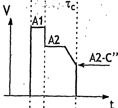
U switch pixel signal FIG.8d
