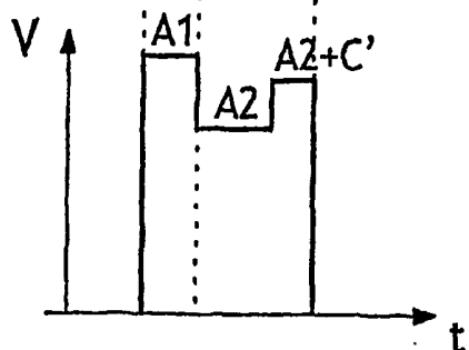
T switch pixel signal FIG.7e
