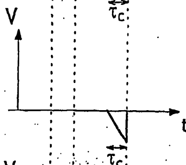
T switch column signal FIG.8c
