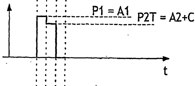
T switch pixel signal FIG.6e
