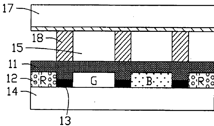
FIG. 8 (PRIOR ART)
