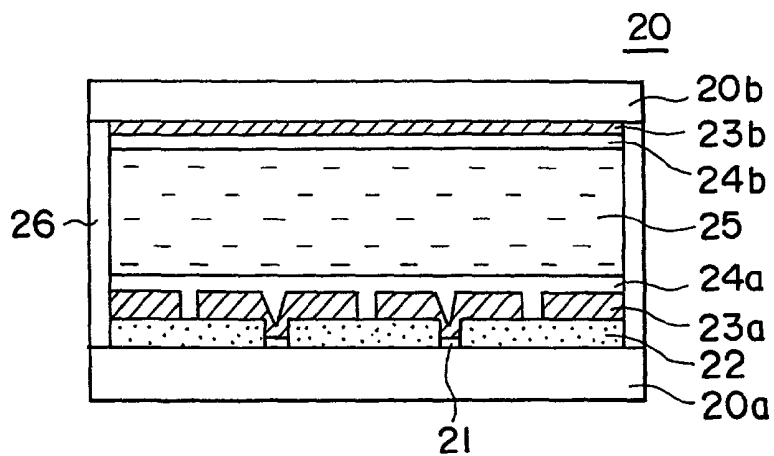
FIG.15 PRIOR ART
