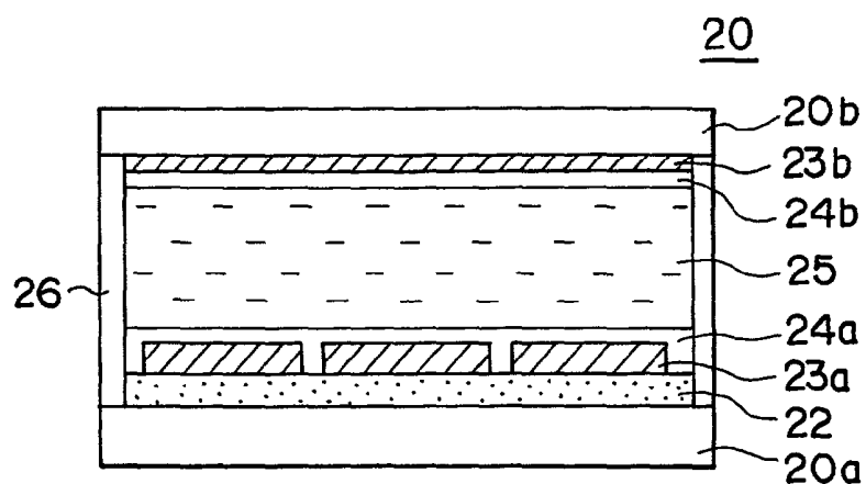
FIG.14 PRIOR ART
