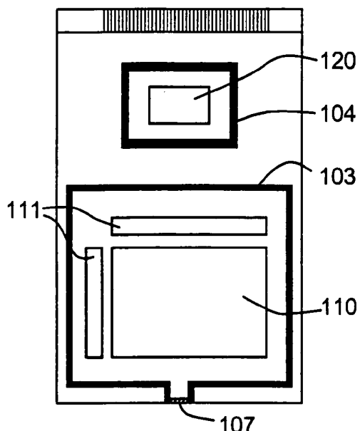
SEALING STRUCTURE OF THE PRESENT INVENTION
