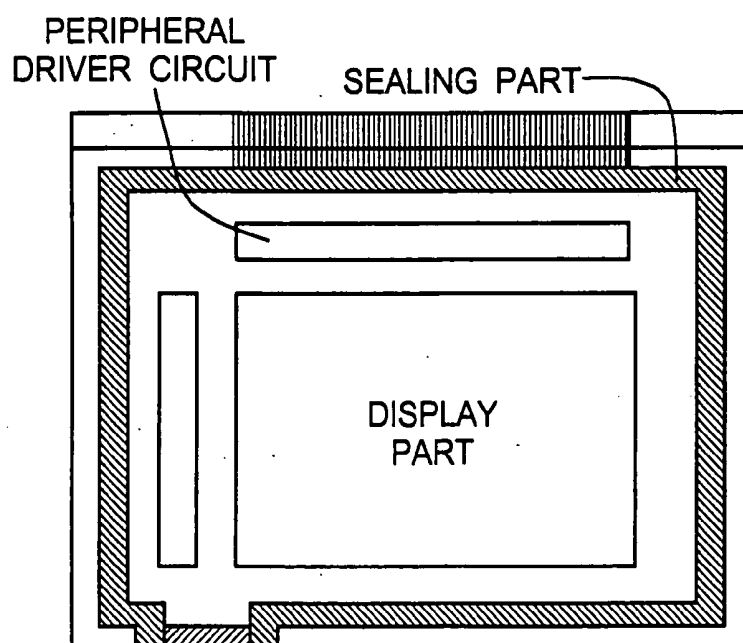
STRUCTURE OF CONVENTIONAL PANEL
