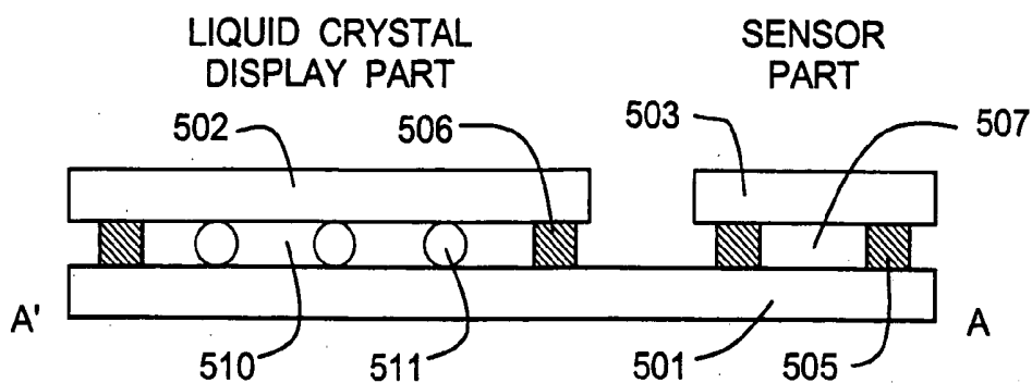
CROSS SECTIONAL VIEW TAKEN ALONG LINE A - A'
