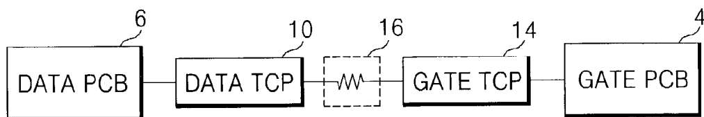
FIG. 3 RELATED ART
