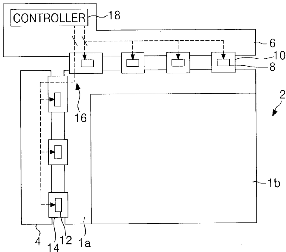
FIG. 1 RELATED ART
