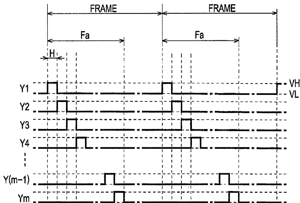
FIG. 5A SCANNING LINE DRIVING CIRCUIT
