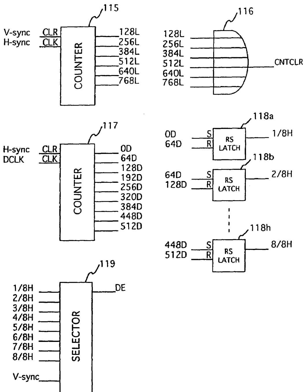
FIG. 40 DYNAMIC RANGE DESIGNATING PORTION
