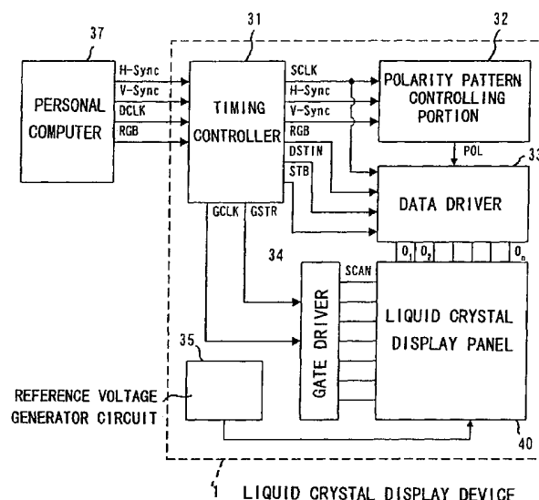
CONFIGURATION OF LIQUID CRYSTAL DISPLAY DEVICE
