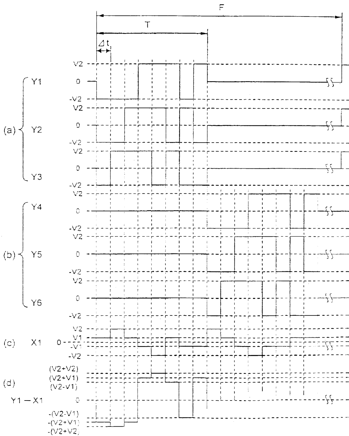
FIG. 13 PRIOR ART
