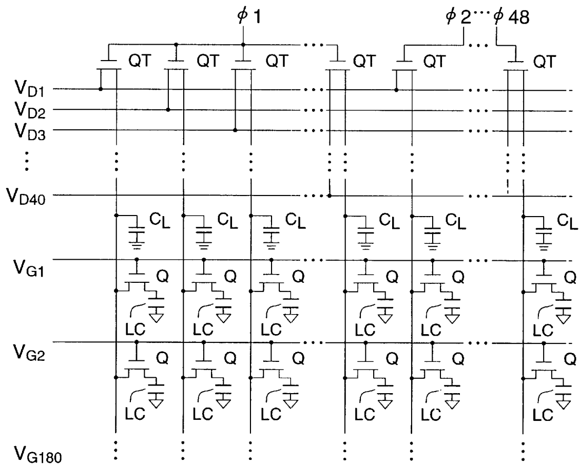
FIG. 7 PRIOR ART
