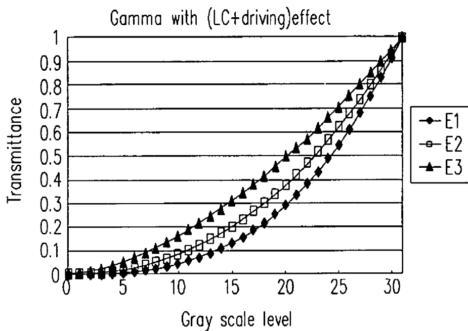
FIG. 5 (PRIOR ART)
