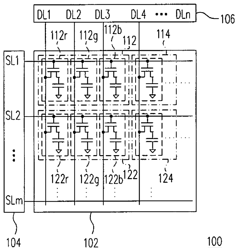
FIG. 1 (PRIOR ART)
