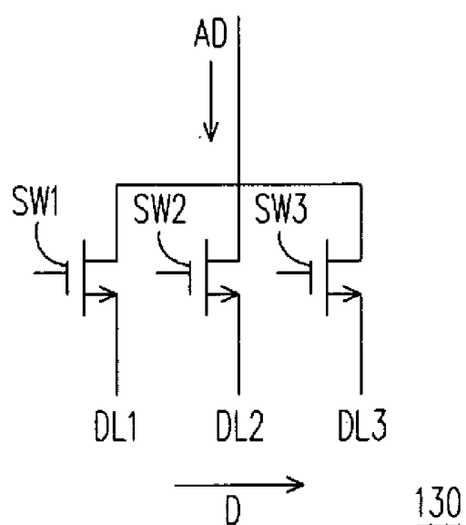
FIG. 3 (PRIOR ART)
