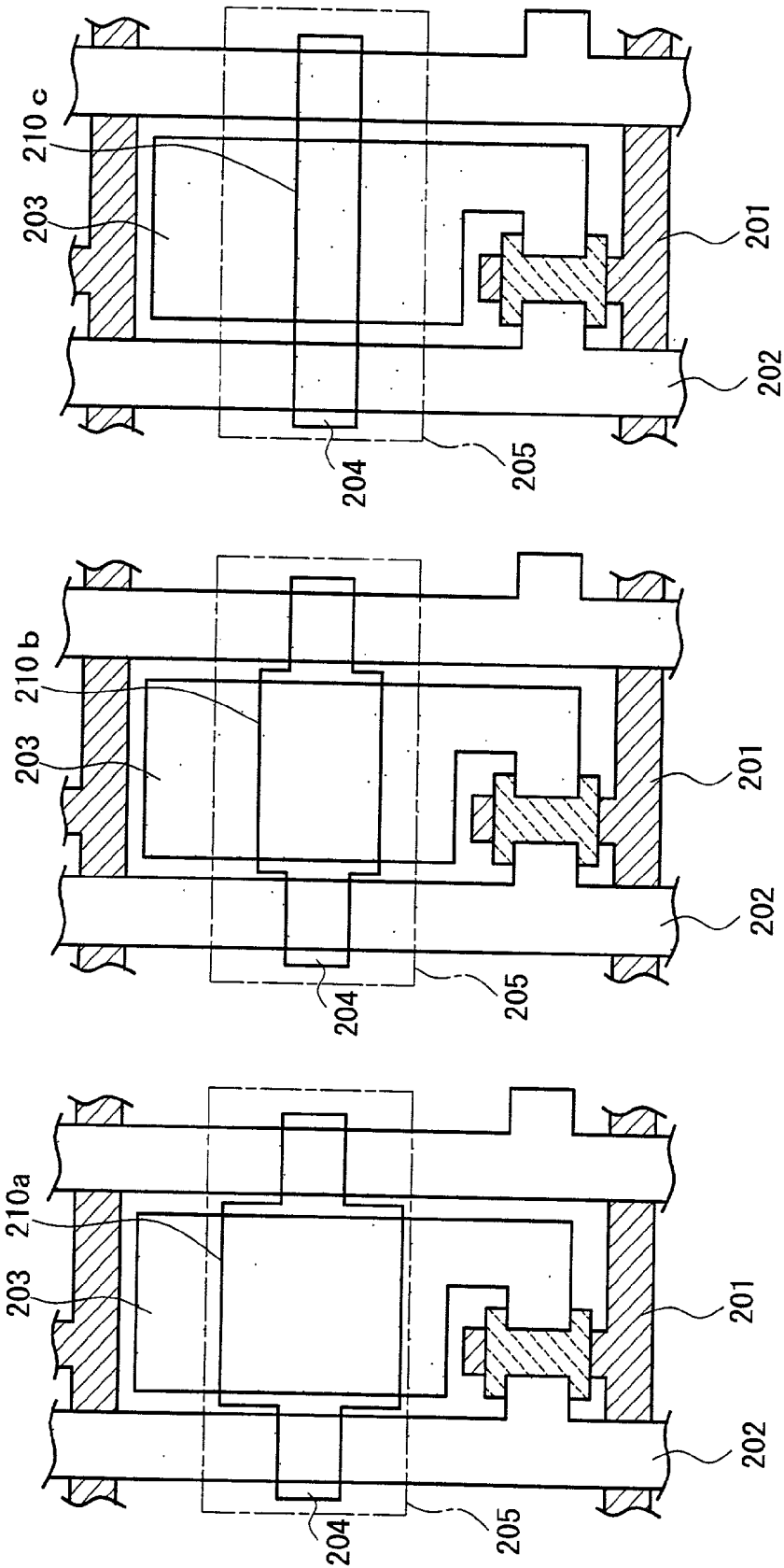
FIG. 38C (PRIOR ART)
