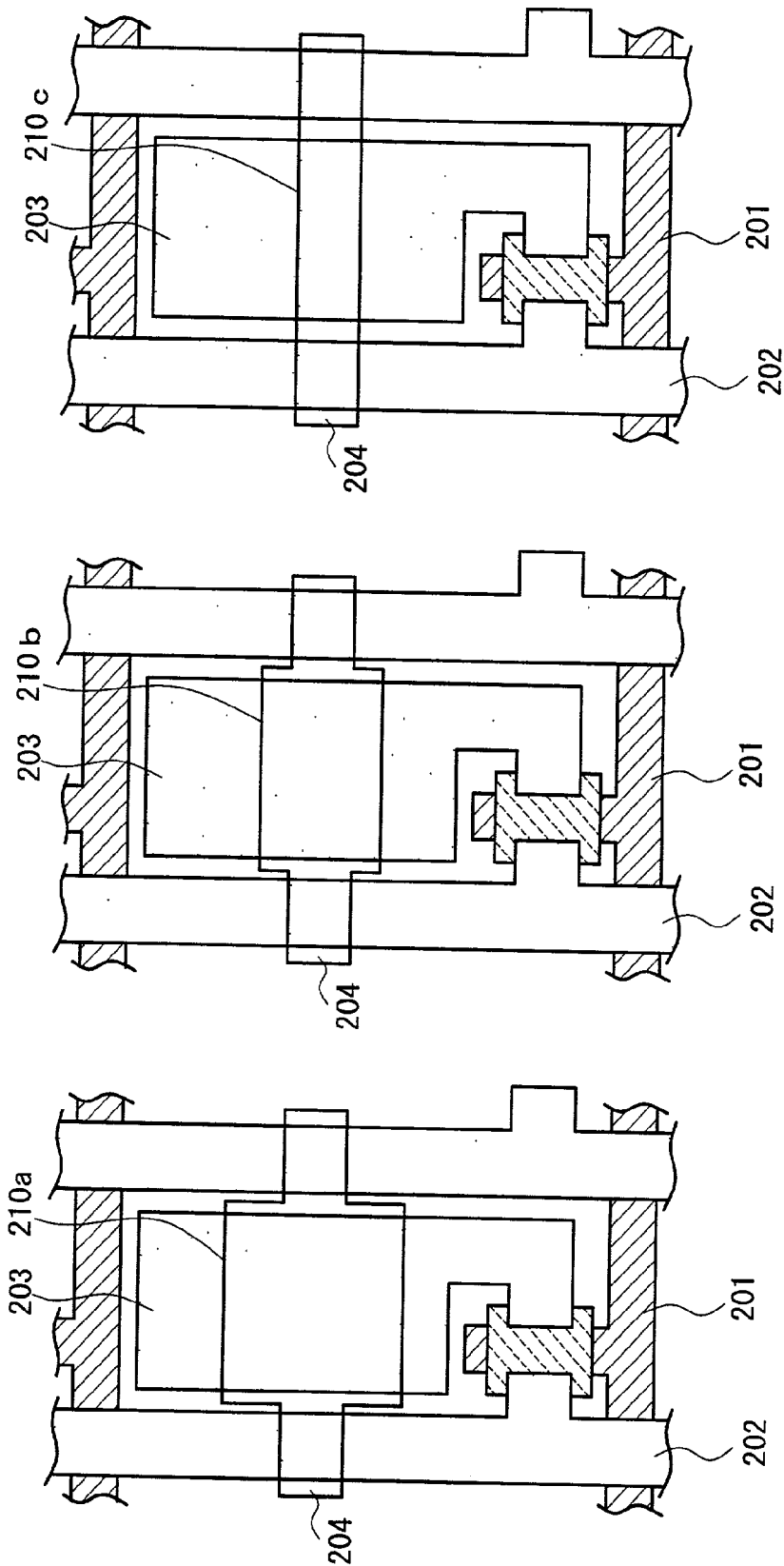
FIG. 37A (PRIOR ART)
