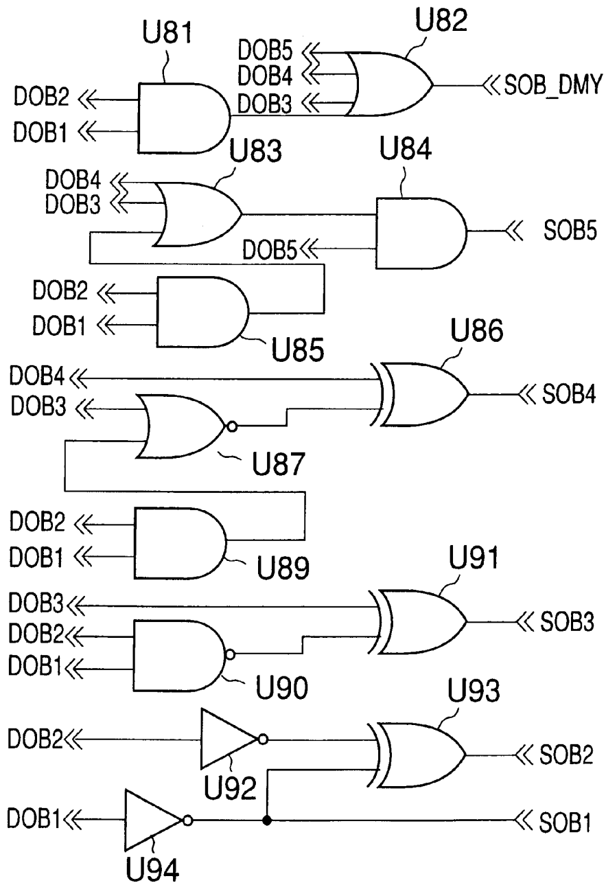
6-steps gradation subtraction circuit
