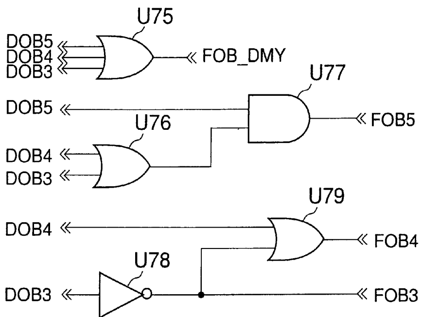
8-steps gradation subtraction circuit
