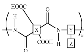
[Chem 2]
