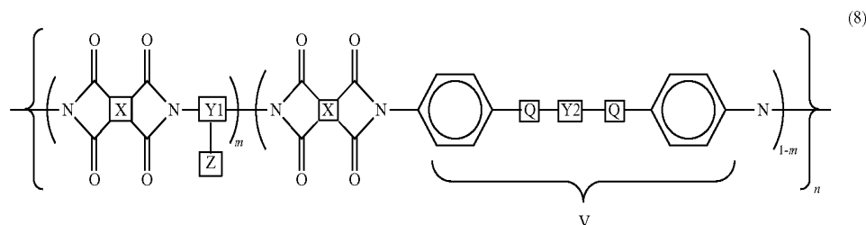
[Chem 8]
