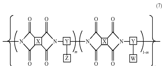
[Chem 7]
