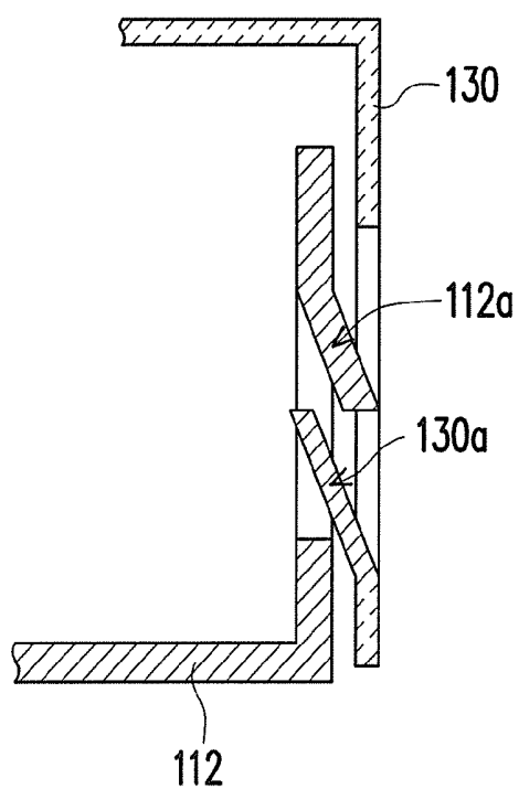
FIG. 2A(PRIOR ART)
