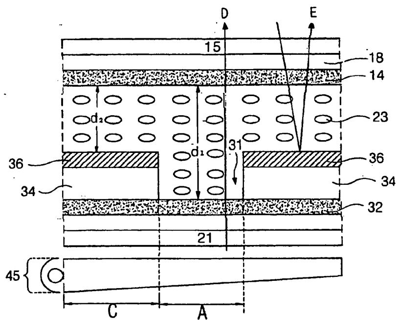
(related art) FIG. 2
