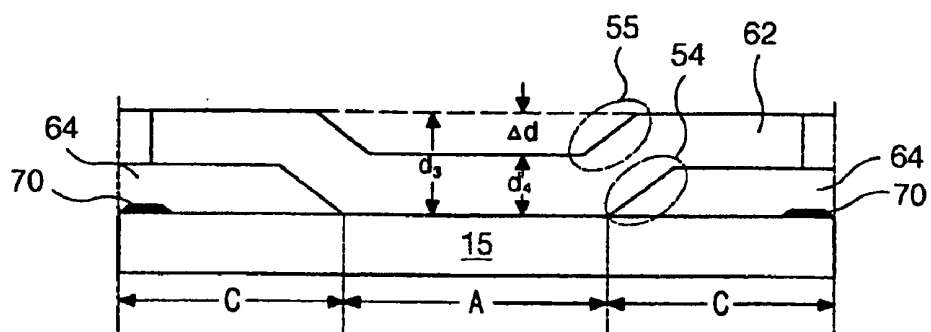
(related art) FIG. 5B
