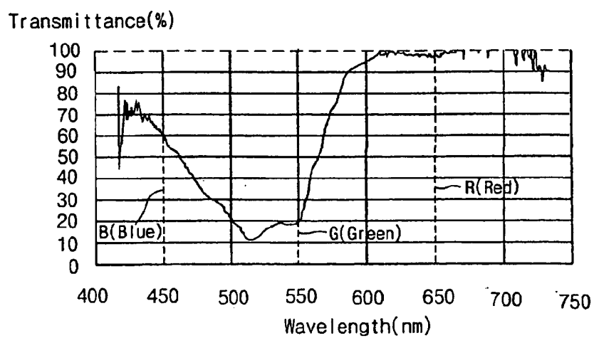
(related art) FIG. 3A
