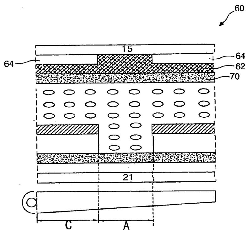
(related art) FIG. 3B
