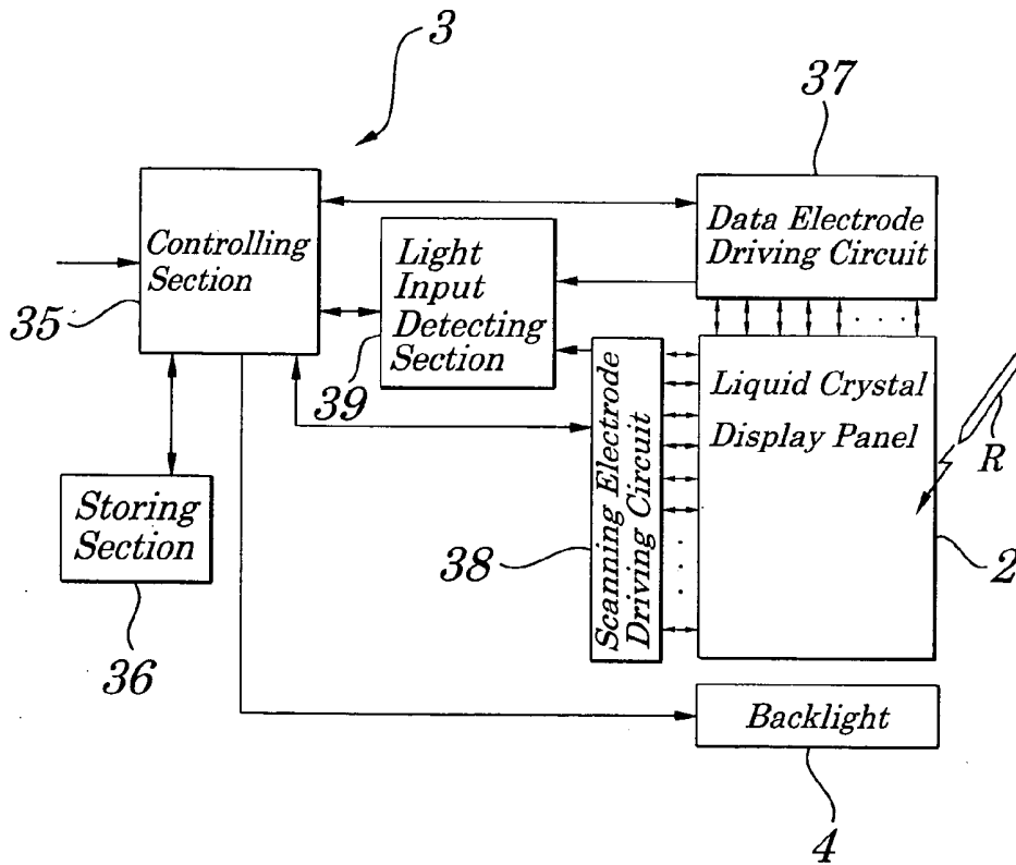
1 ; Liquid Crystal Display Device
