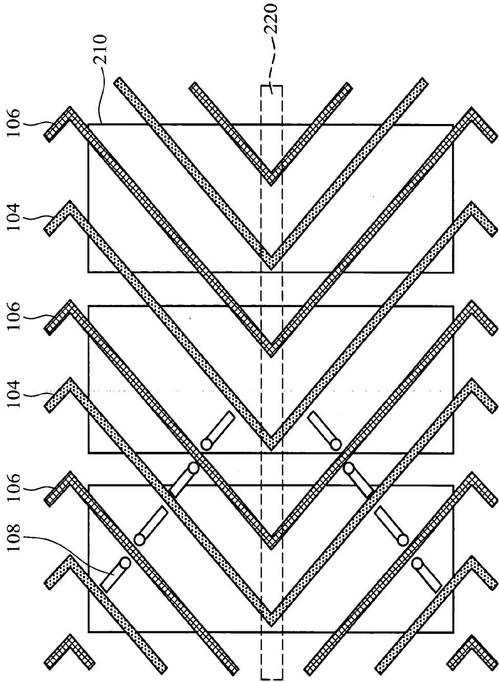
FIG. 2 (RELATED ART)
