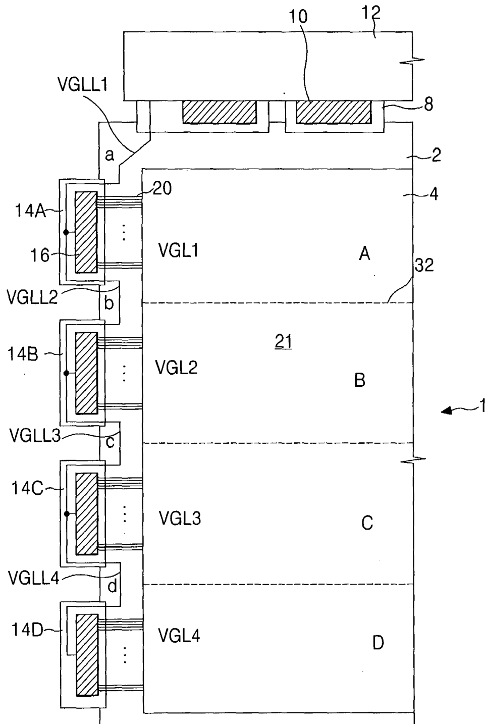
FIG. 2 RELATED ART
