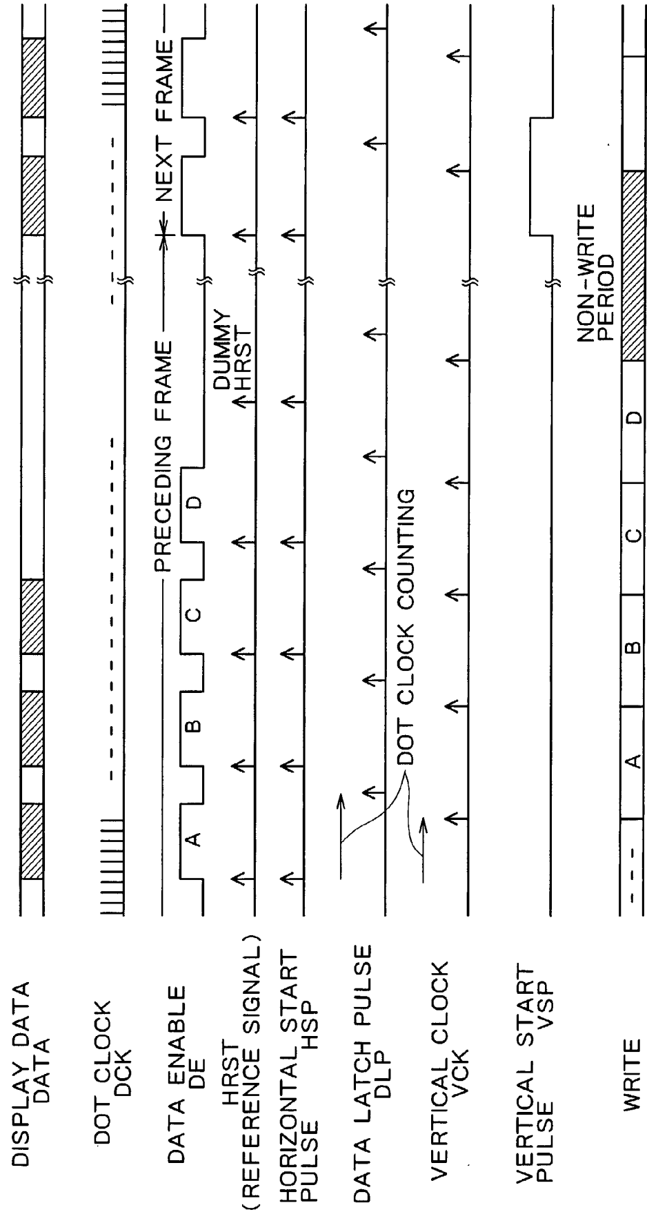
FIG. 2 (PRIOR ART)
