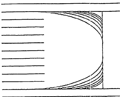
Field 'OFF' State Planar aligned LC
