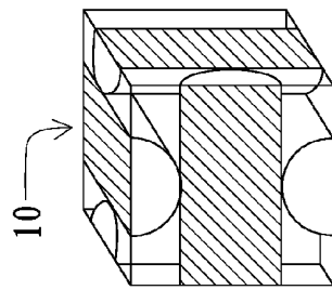
FIG. 1c (Prior Art)
