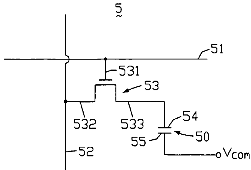
FIG. 5 (RELATED ART)
