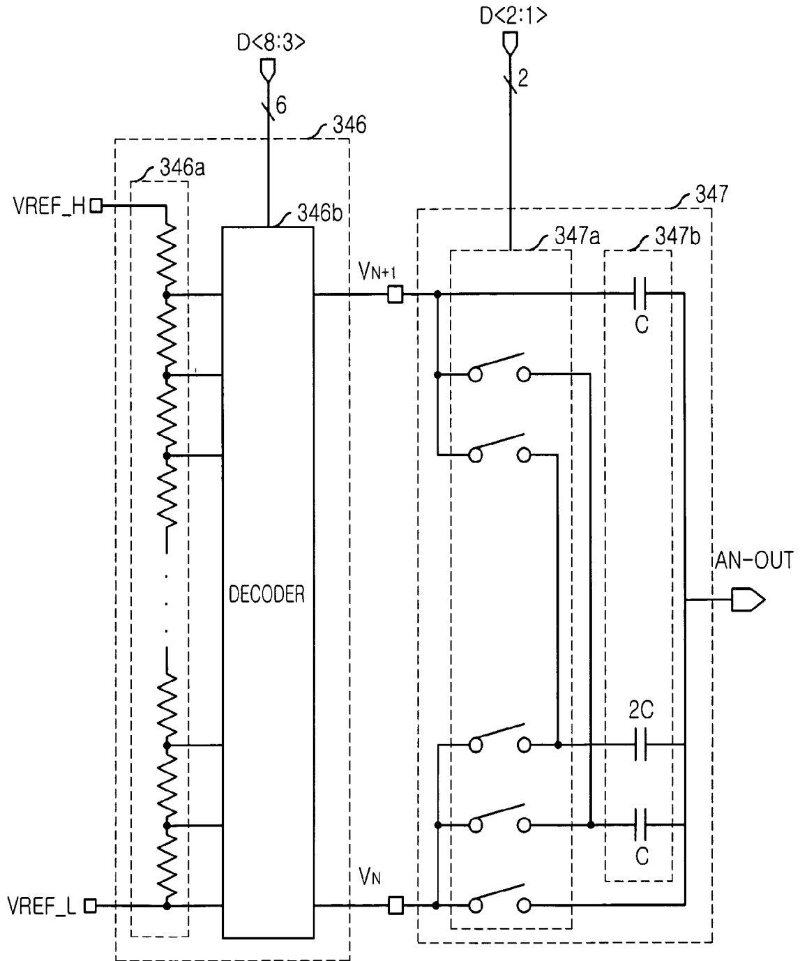
FIG. 5 (PRIOR ART)
