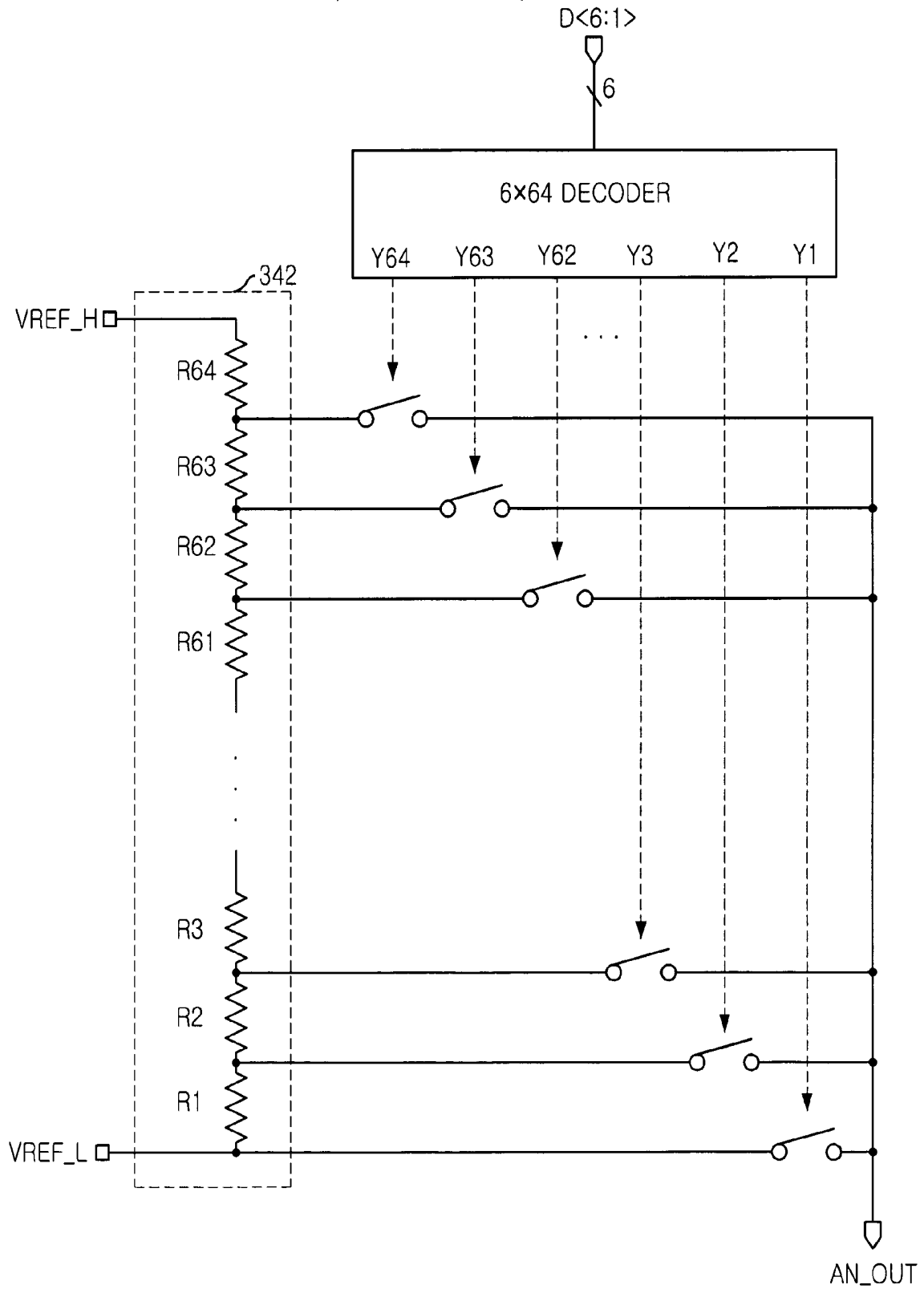
FIG. 4 (PRIOR ART)
