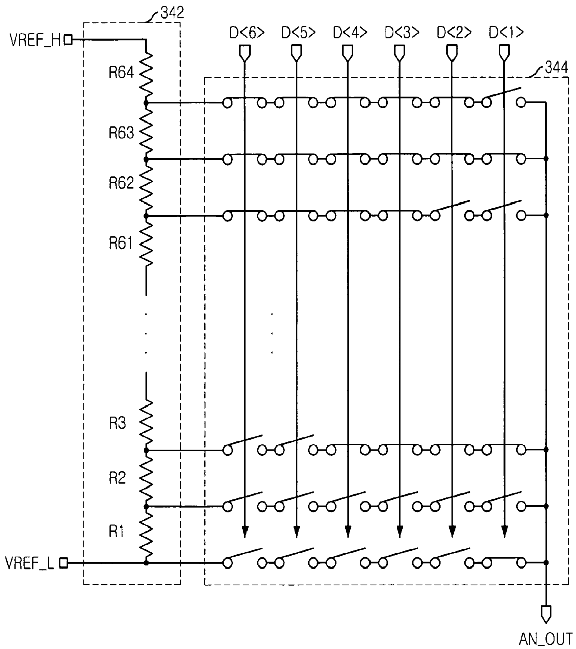
FIG. 3 (PRIOR ART)
