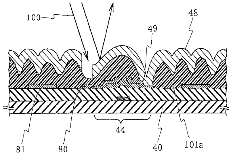
FIG. 13(a) REFLECTIVE LIQUID CRYSTAL DISPLAY APPARATUS
