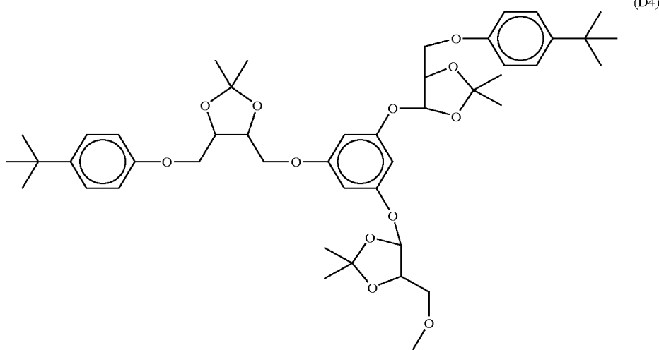
dendrimer skeleton (star-burst type compound)
