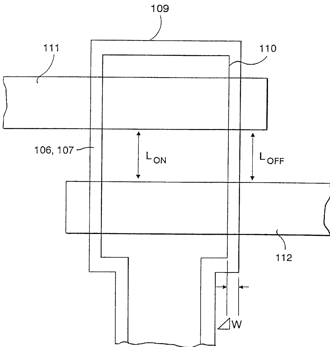
Figure 8 PRIOR ART
