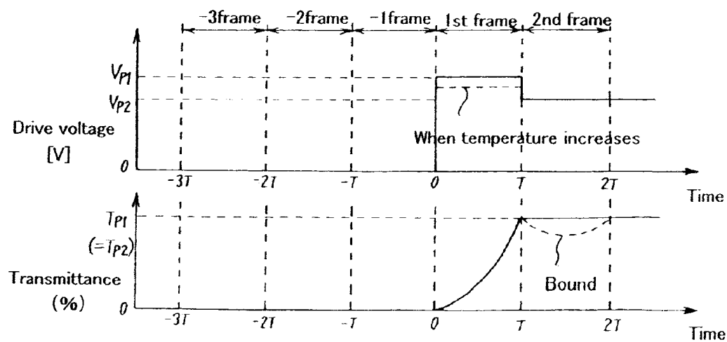
FIG. 20C With Compensation
