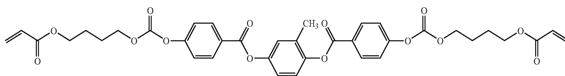
Structural Formula (1)
