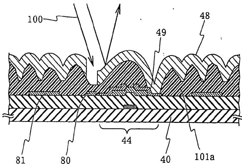
FIG. 13(a) REFLECTIVE LIQUID CRYSTAL DISPLAY APPARATUS
