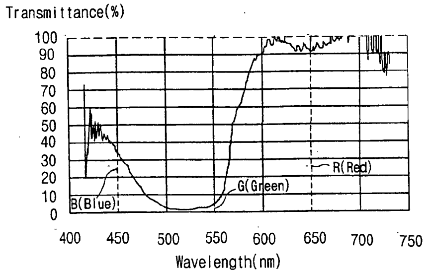
(related art) FIG. 3B
