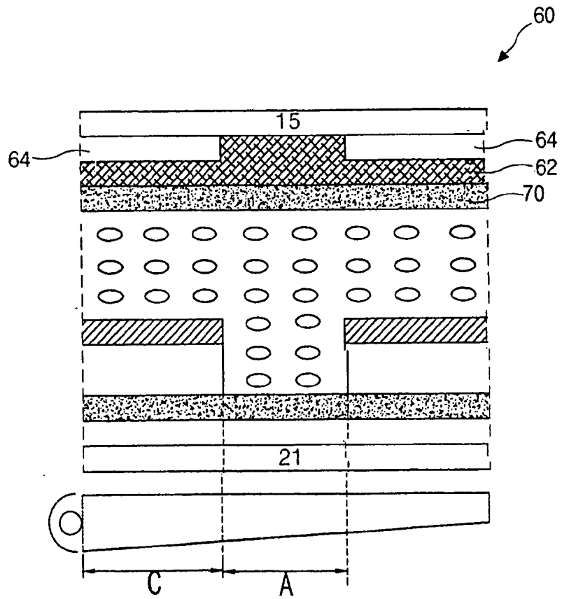
(related art) FIG. 3B
