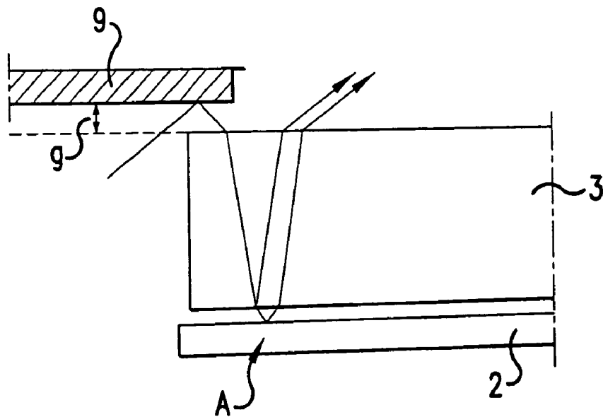
FIG. 2 CONVENTIONAL ART
