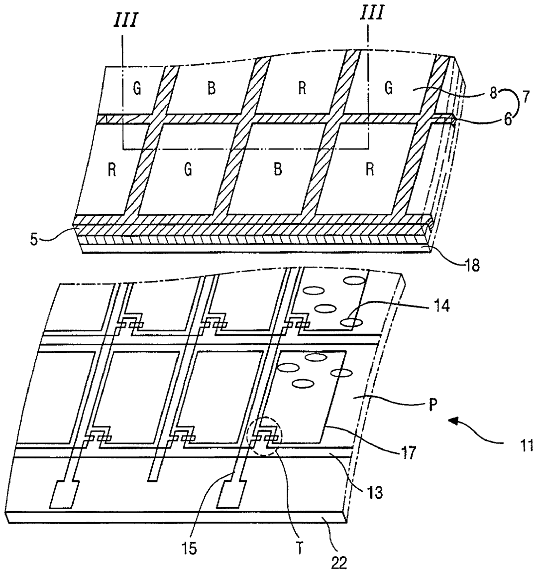
FIG. 1 (RELATED ART)
