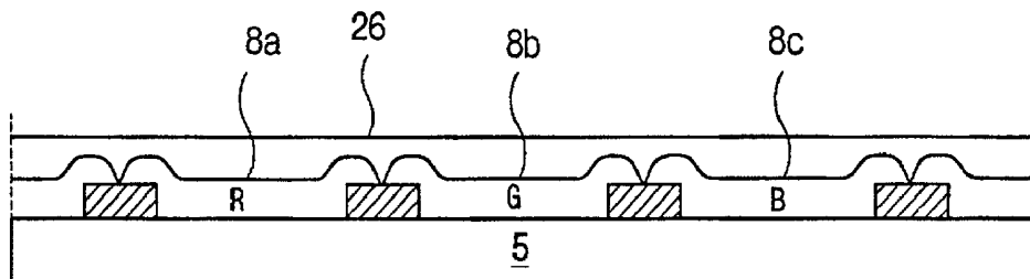
FIG. 3C (RELATED ART)
