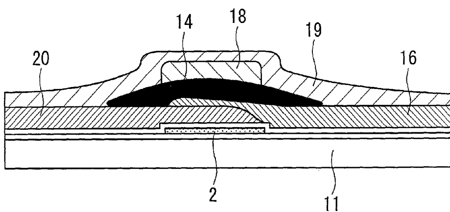
FIG. 5 (CROSS SECTION ALONG B-B)
