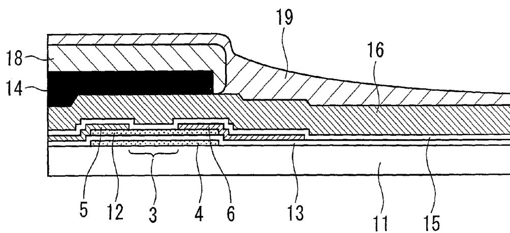
FIG. 4 (CROSS SECTION ALONG A-A)
