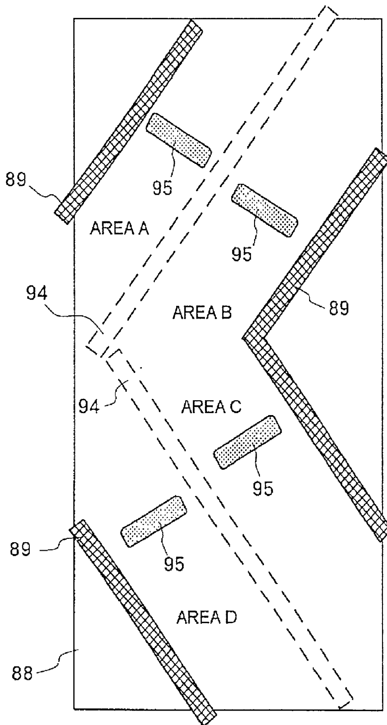
FIG. 2 (PRIOR ART)
