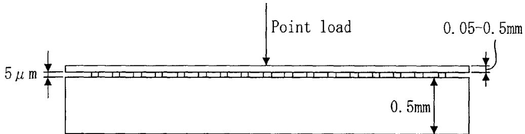
FIG. 14 PRIOR ART
